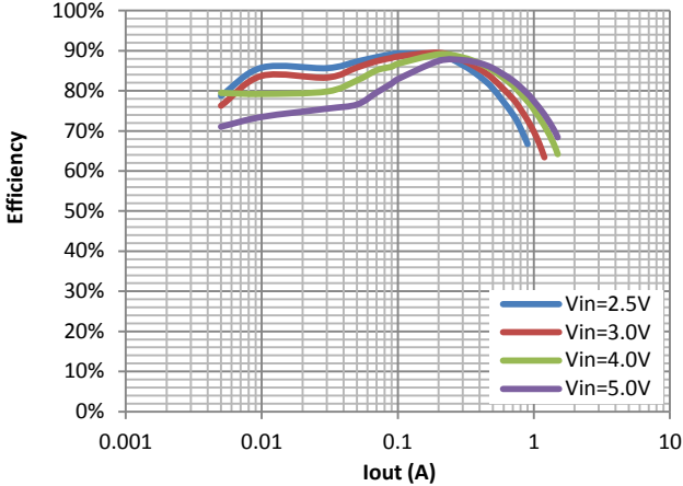
Efficiency vs. Output Current ( V_{out}=1.2\text{V} )
