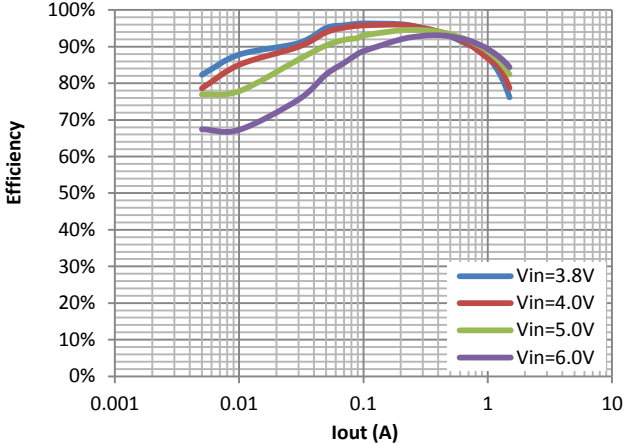
Efficiency vs. Output Current ( V_{out}=3.3\text{V} )
